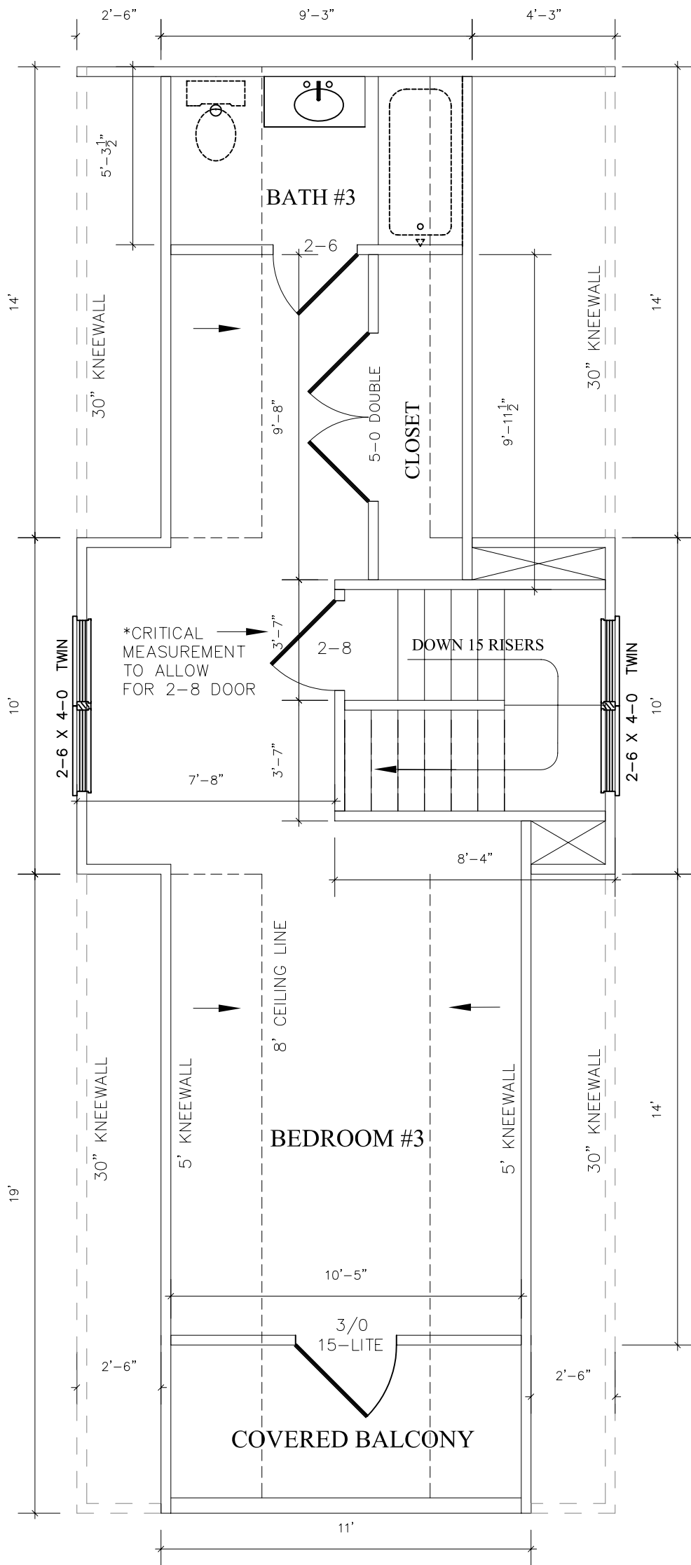
16' SHOTGUN 3RD FLOOR PLAN
