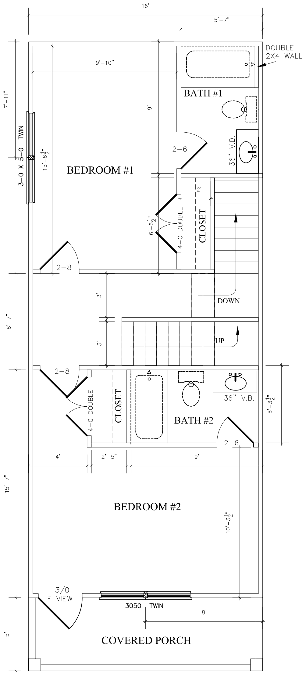
2.16 16' SHOTGUN 2ND FLOOR PLAN SCALE 1/4" = 1'
