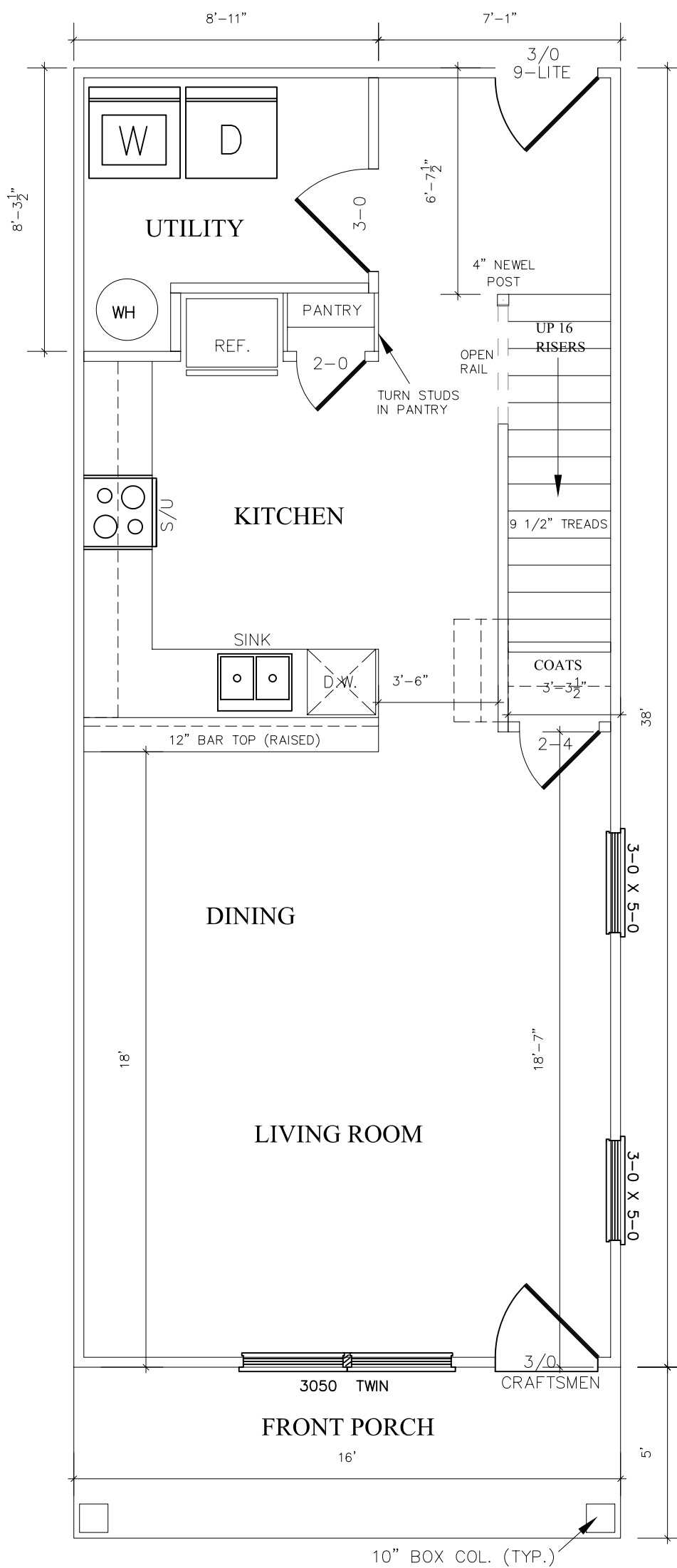
1.16 16' SHOTGUN 1ST FLOOR PLAN SCALE 1/4" = 1'
